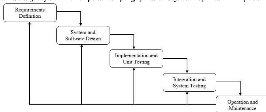
Gambar 6. Metode Waterfall
